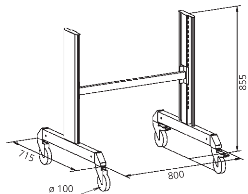
Fitter's trolley 4
