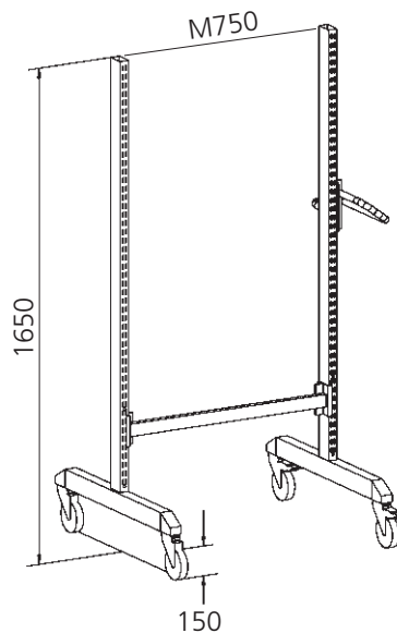
Basic trolley frame
